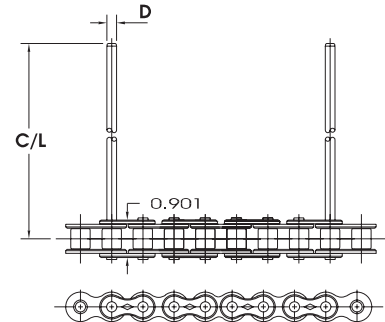
STANDARD PIN OVEN CHAIN 标准制罐运输链
